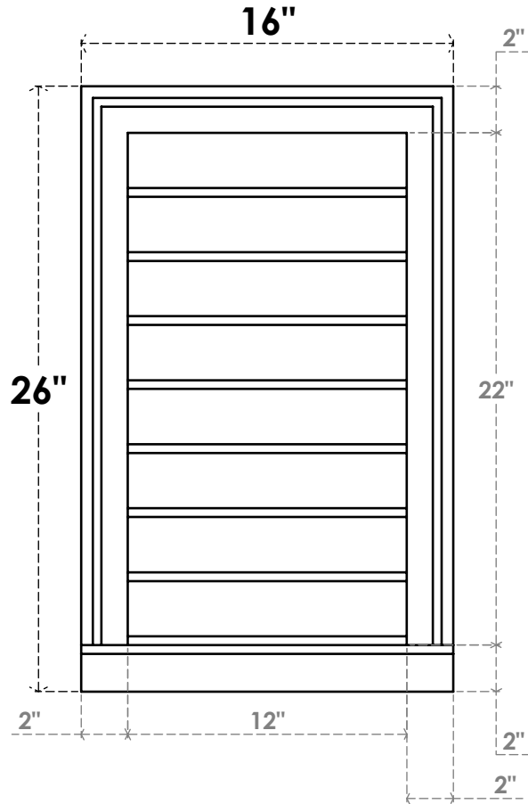
FRONT
